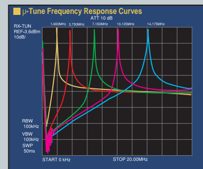
10dB/Div - 2 MHz/Div
