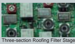
Three-section Roofing Filter Stage
