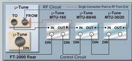
RF \mu -Tuning Kit Connection Diagram
